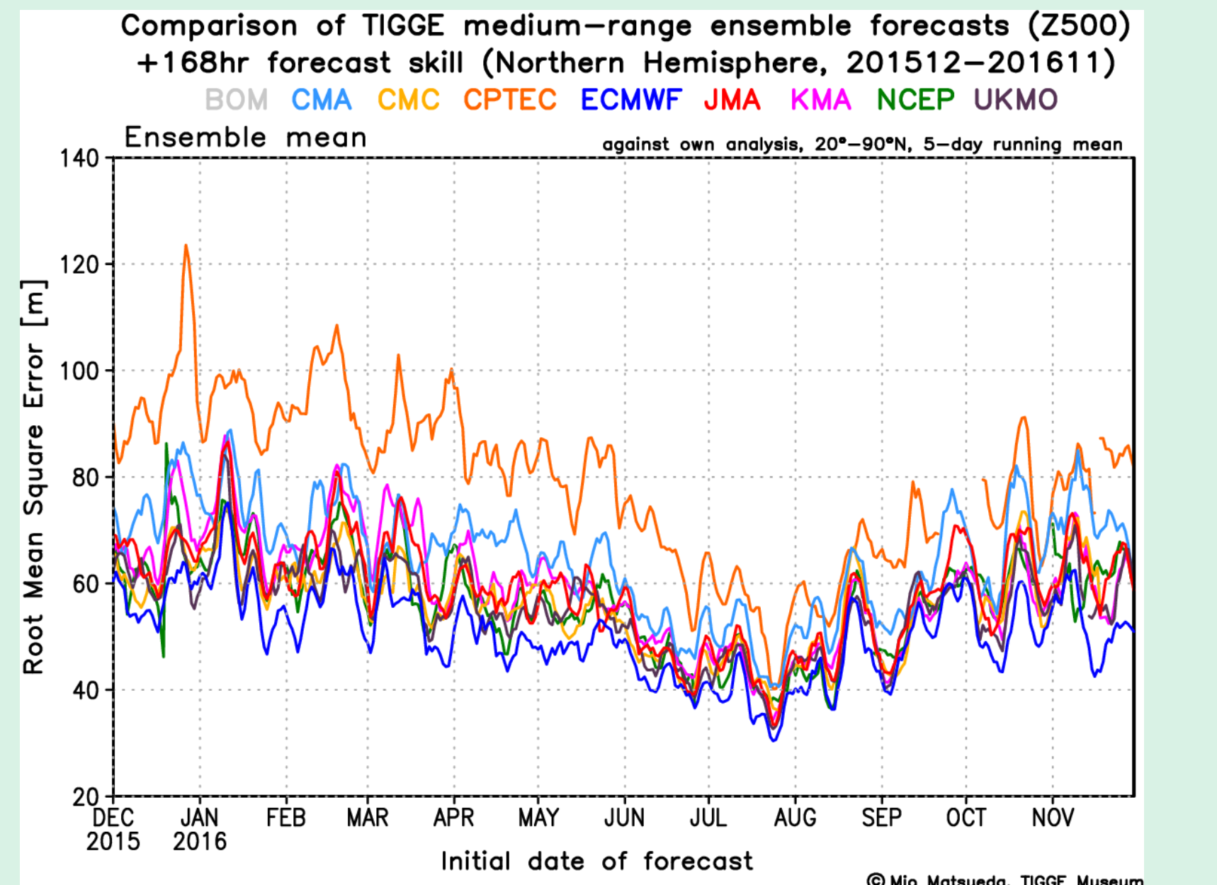
Figure 4: Root Mean Square Error (RMSE) for 7-day ensemble mean forecasts of 500 hPa height (Z500) over the Northern Hemisphere, initialised in December 2015 – November 2016. Each forecast is verified against its own analysis.
