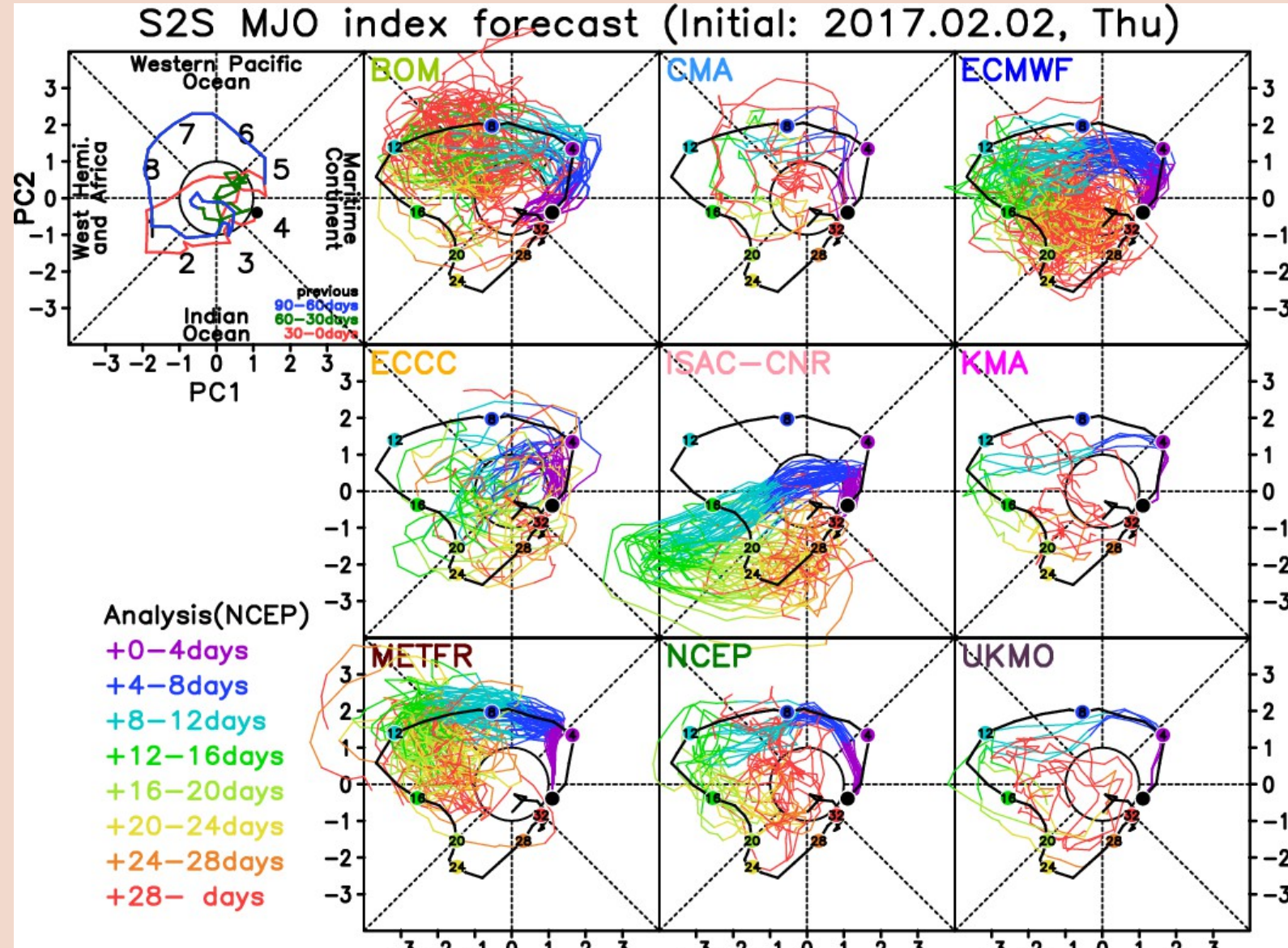
Figure 7: (top left) NCEP control analysis for real-time multivariate MJO index for the 90 days prior to the initial date of the forecast. (right 9 panels) Real-time multivariate MJO index forecasts by BoM, CMA, ECMWF, ECCC, ISAC-CNR, KMA, METFR, NCEP, and UKMO, initialised on 2 February 2017. The black circle and the black line with numbered circles correspond to the NCEP control analysis. The numbers in the coloured circles indicate the number of days from the initial date. The coloured lines indicate ensemble members. The colour changes reflect the lead-time of the forecasts.
