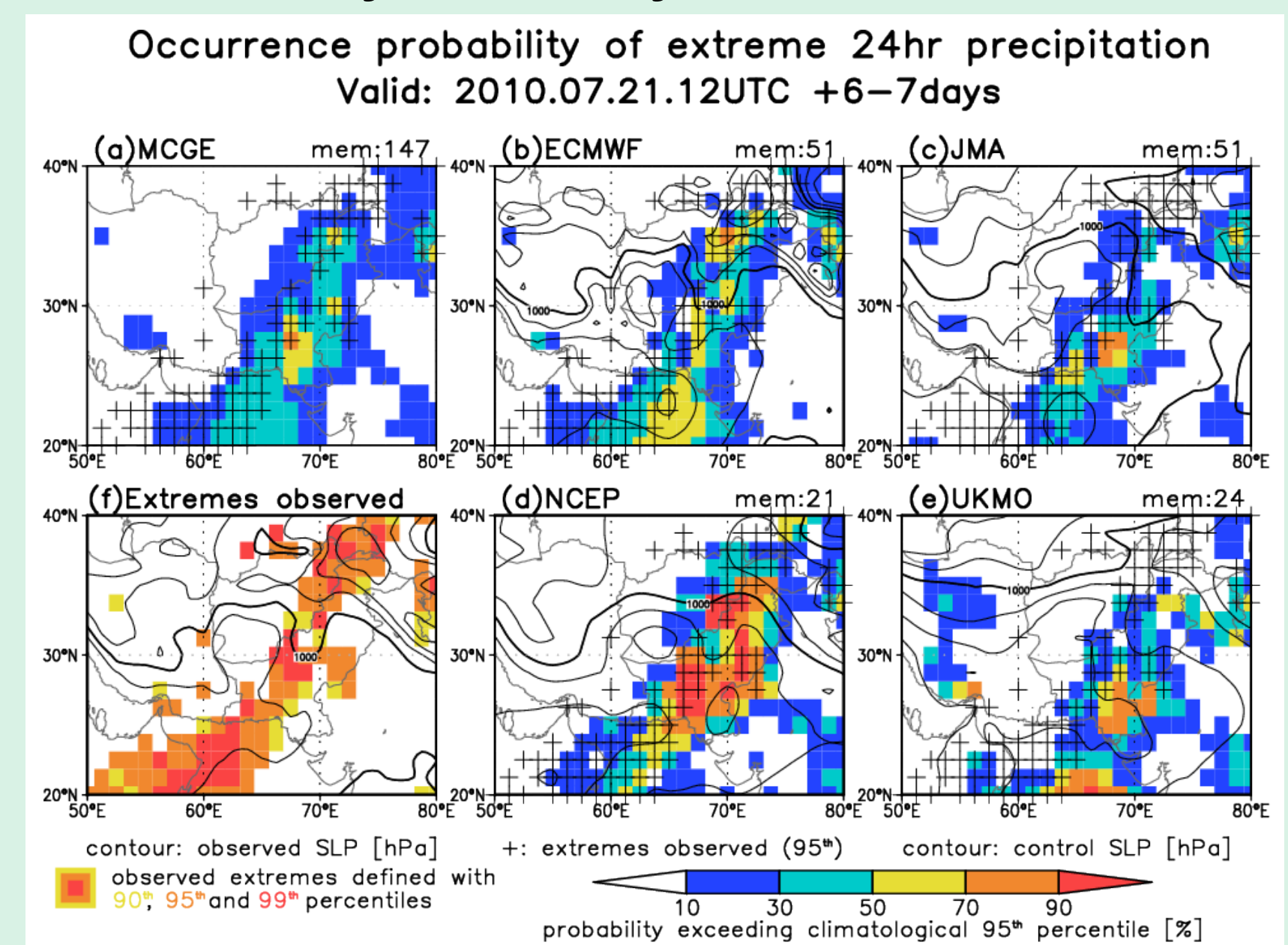
Figure 3: Occurrence probabilities of extreme 24-hr rainfall for the 2010 Pakistan floods. The shading indicates occurrence probabilities by the (a) multicentre grand ensemble, (b) ECMWF ensemble, (c) JMA ensemble, (d) NCEP ensemble, and (e) UKMO ensemble, initialised at 1200UTC 21 July 2010, and valid at 1200UTC 27 – 28 July 2010. Contours in (b–e) indicate predicted sea level pressure (SLP) in each control run. (f) Observed extremes defined with the observed climatological 90th, 95th and 99th percentiles (shading) and SLP (contours). The hatching in (a–e) indicates observed extremes defined with the observed 95th percentiles in (f). The climatological 95th percentiles of the models were used to define the predicted extremes. (Matsueda and Nakazawa, Meteorol. Appl., 2015)
