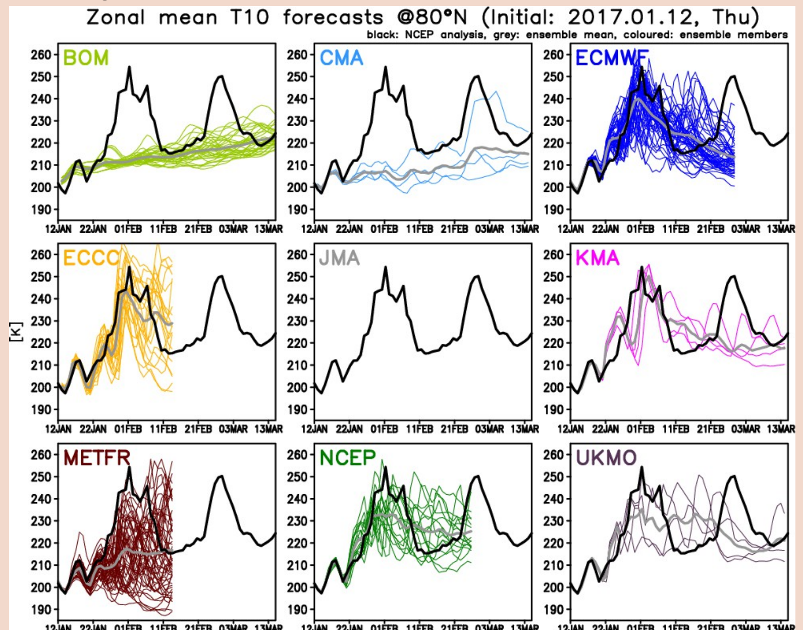
Figure 6: Zonal mean temperature at 10 hPa over 80°N line forecasts by BoM (yellow-green), CMA (aqua), ECMWF (blue), ECCC (yellow), KMA (pink), METFR (brown), NCEP (green), and UKMO (purple), initialised on 12 January 2017. The coloured and grey lines indicate individual ensemble members and ensemble mean, respectively. The black line corresponds to the NCEP control analysis.
