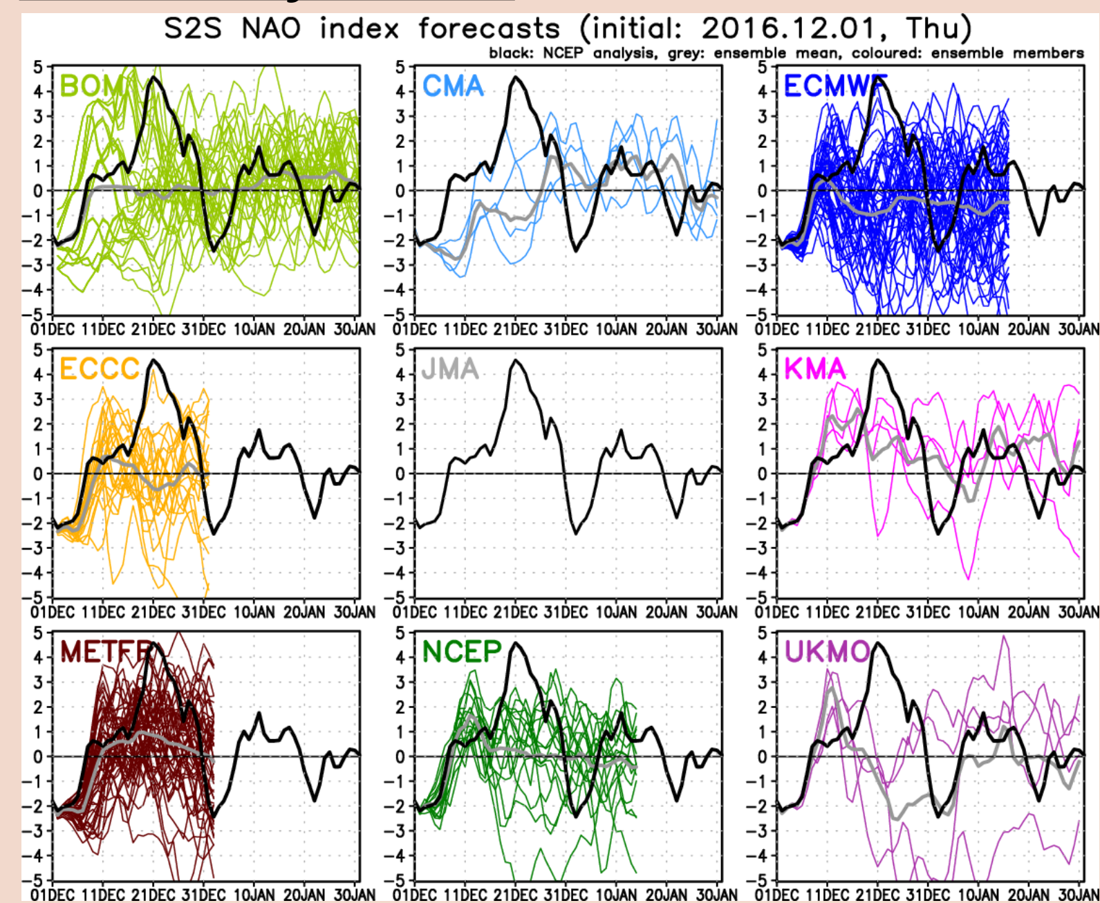
Figure 5: NAO index forecasts by BoM (yellow-green), CMA (aqua), ECMWF (blue), ECCC (yellow), KMA (pink), METFR (brown), NCEP (green), and UKMO (purple), initialised on 1 December 2016. The coloured and grey lines indicate individual ensemble members and ensemble mean, respectively. The black line corresponds to the NCEP control analysis.
