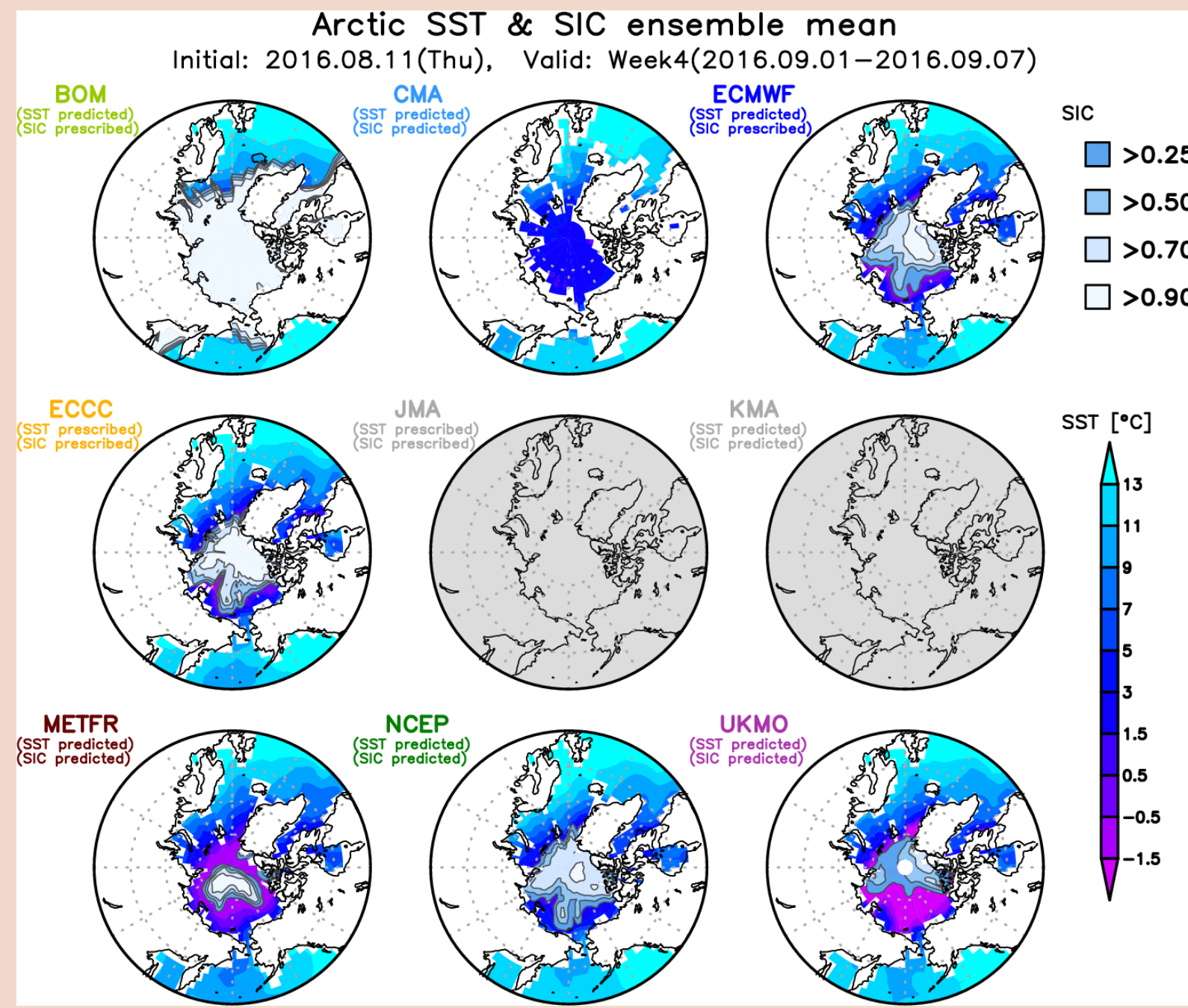
Figure 8: Sea surface temperature (colour bar at the lower-right corner) and sea ice cover (colour bar at the upper-right corner) forecasts by BoM (yellow-green), CMA (aqua), ECMWF (blue), ECCC (yellow), METFR (brown), NCEP (green), and UKMO (purple), initialised on 11 August 2016, valid on 1 – 7 September 2016 (Week 4).
